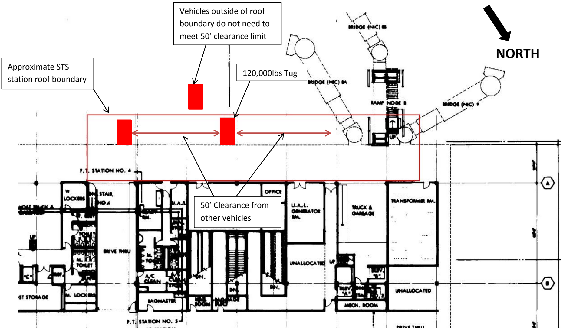
Figure 1: Parking Limits at North Satellite Apron
